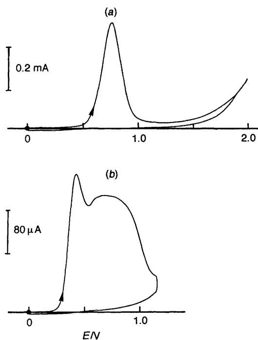
Fig. 5 Cyclic voltammograms (anodic region) of [(CuL^1)_2] (a) and [(CuL^2)_2] (b), 3.7 mmol dm -3 , in MeCN + 0.1 mol dm -3 NBu_4ClO_4 at a platinum electrode (5 mm diameter); scan rate 0.1 V s -1 ; E vs. Ag-10 mmol dm -3 AgNO_3 + MeCN + 0.1 mol dm -3 NBu_4ClO_4
